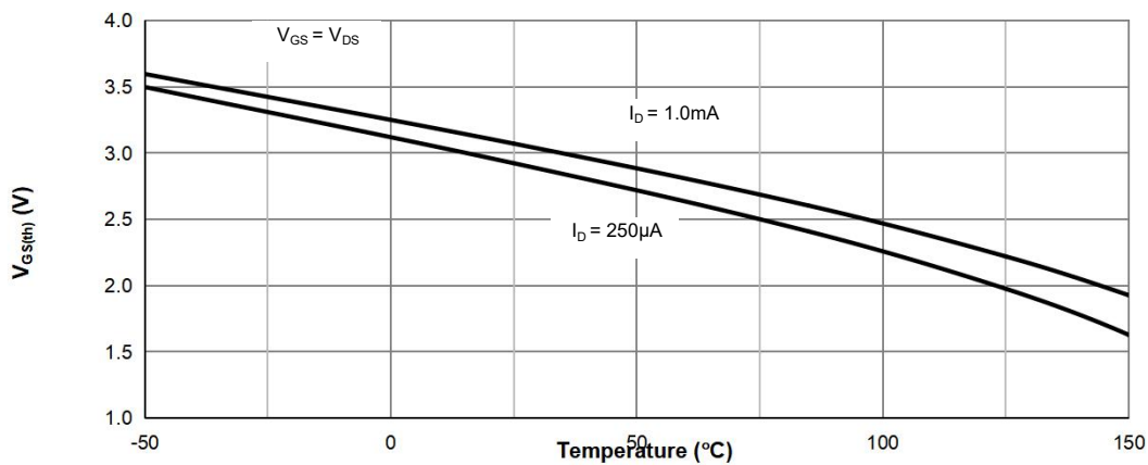
Figure 5: V_{GS(th)} vs. Junction Temperature
